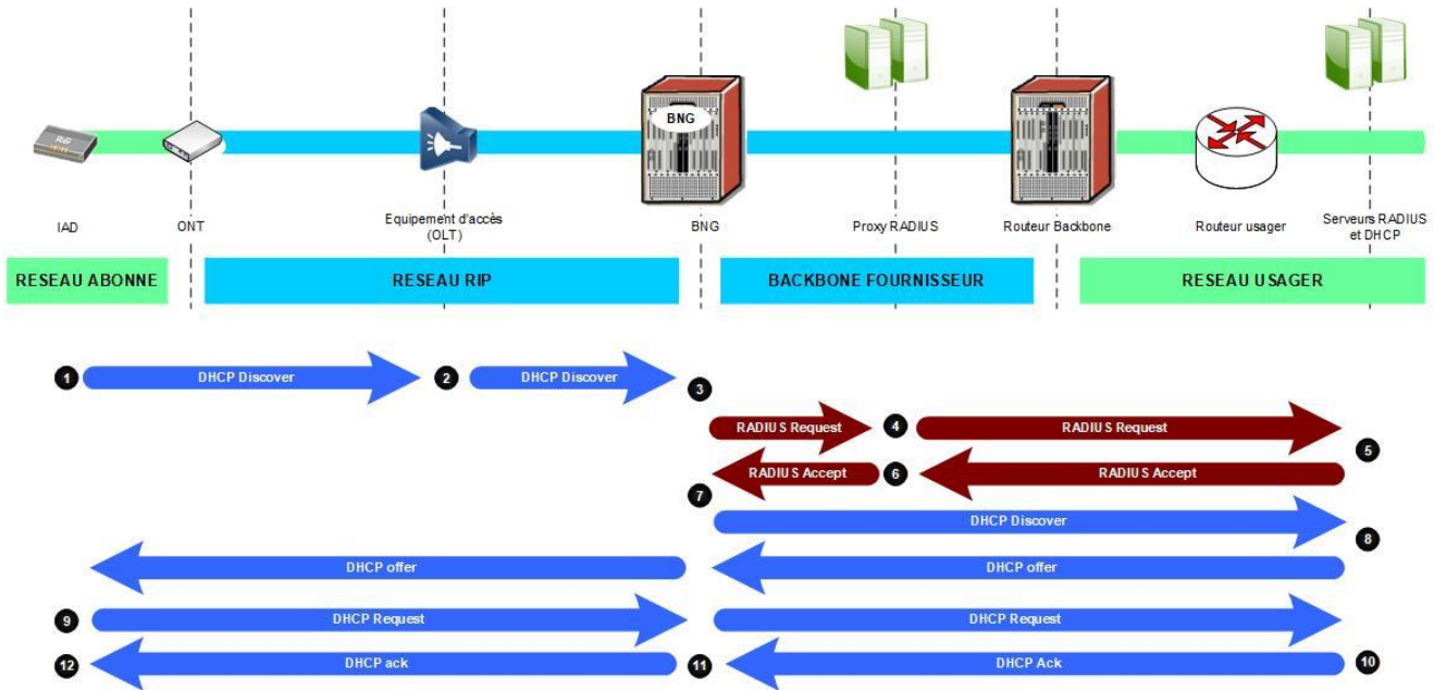
Figure 9 - Mode DHCP et RADIUS (transaction DHCPv4-Discover)
